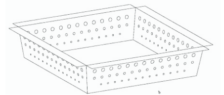
Silt Trap (Stainless Steel) Part No: SILT450
